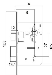
3Lever Mortice Sash Lock
