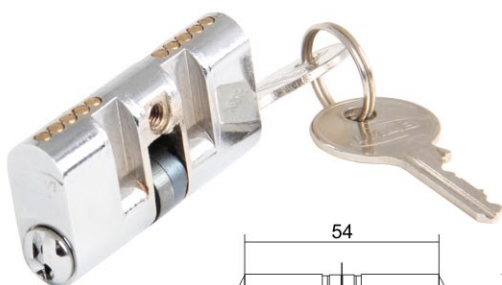
Oval Profile(UK)
