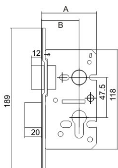
Heavy Duty Euro Sash Lock
