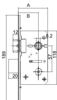
Heavy Duty Bathroom Lock
