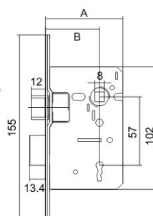
3Lever Mortice Sash Lock Economic
